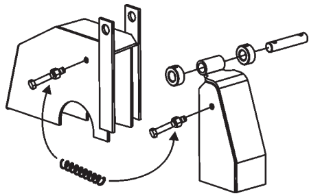
Figure 5. Blade Guard
