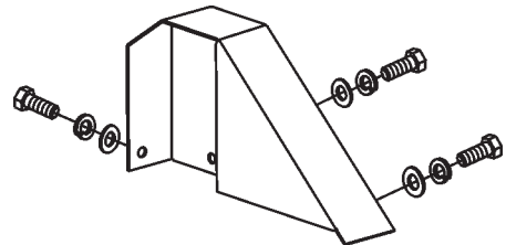
Figure 6. V-Belt Cover
