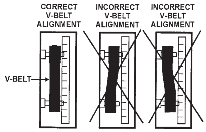
Figure 7. Pulley Alignment
