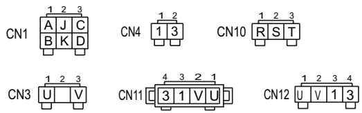
CONNECTOR ARRANGEMENT (WIRING VIEW)
