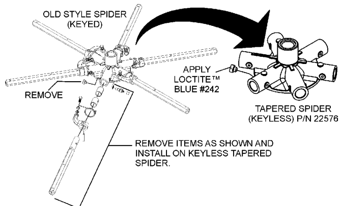
Figure 5. Spider Components
