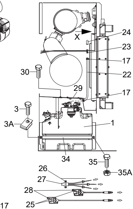
VIEW - X
