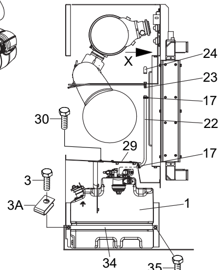
DETAIL - Z
