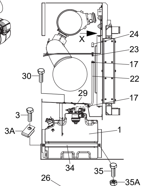
DETAIL - Z
