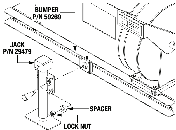
Figure 34. Jack Installation
