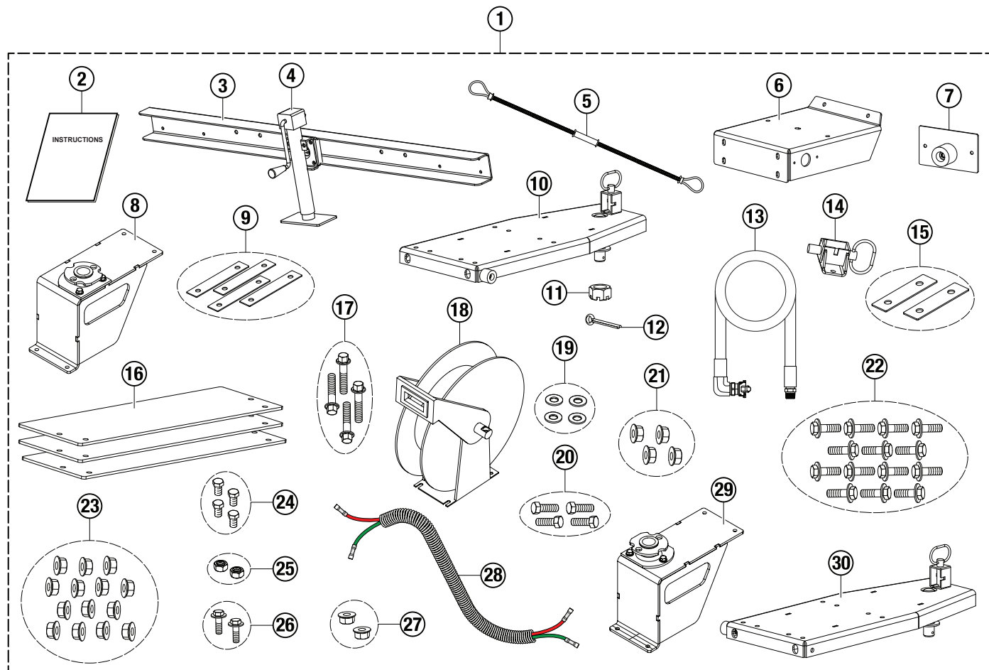
Figure 1. DIS185SSI4F Hose Reel Installation Kit
