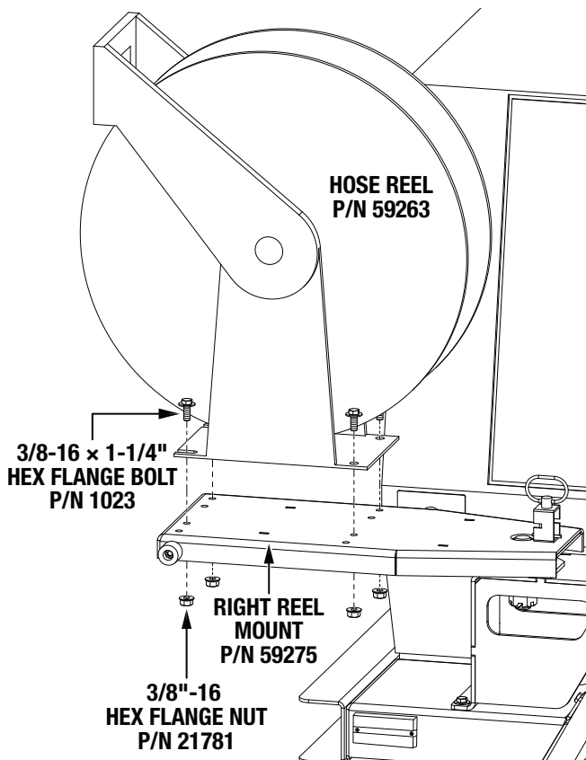
Figure 27. Hose Reel Installation
