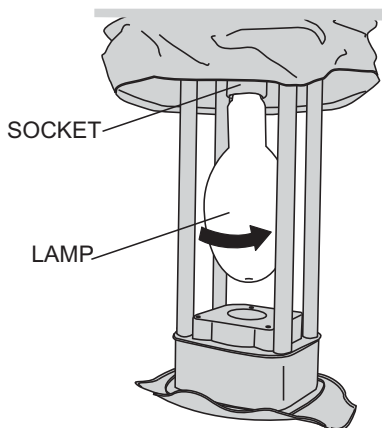
Figure 37. Installing Lamp
