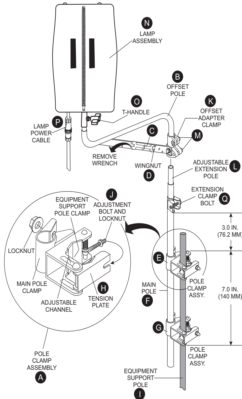
Figure 26. Offset Pole Assembly
