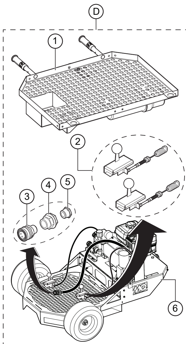
Figure 4. Pallet Contents
